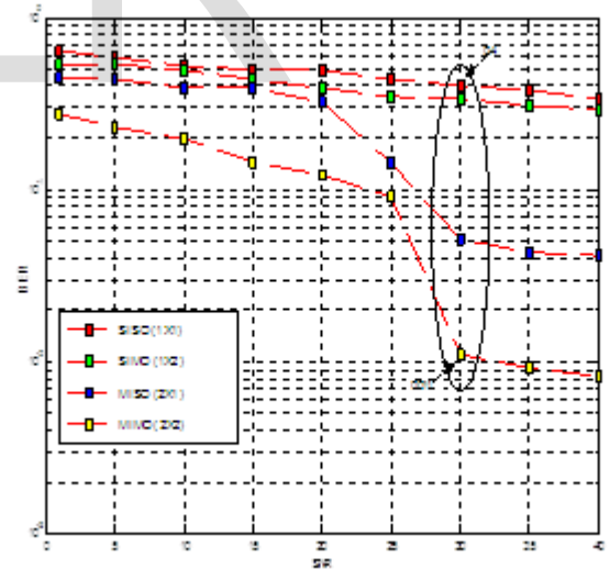
Fig 1: Comparison between SISO, SIMO, MISO, MIMO
