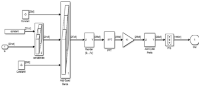
Fig 1(b): OFDM Transmitter
