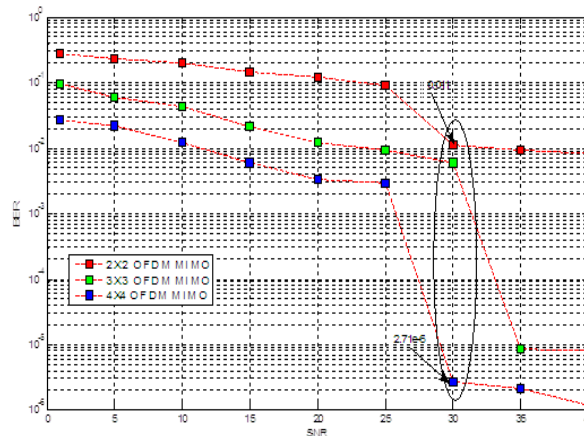
Fig 4: Comparison between 2x2, 3x3, 4x4 OFDM MIMO
