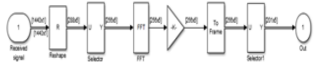
Fig 1(d): OFDM Receiver
