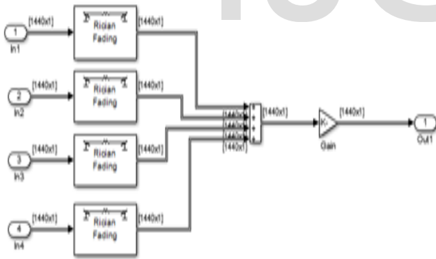
Fig 1(c): MIMO Channel
